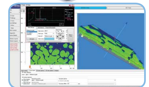
Hydrogen Blistering
