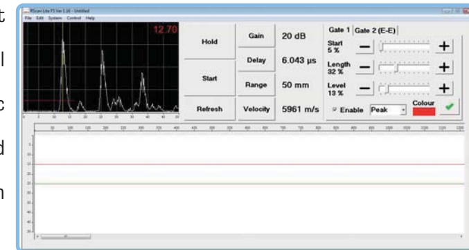
Gain, Time Base Range, Filtering and Gate Settings
