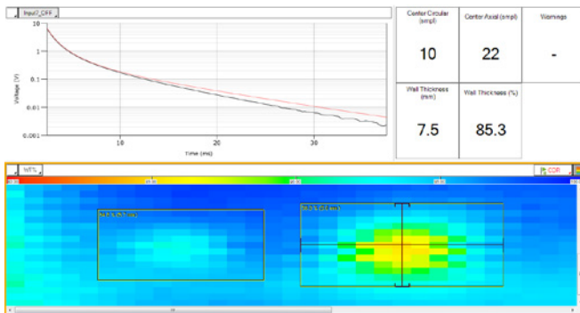
51mm (2in) insulation and aluminum weather jacket
