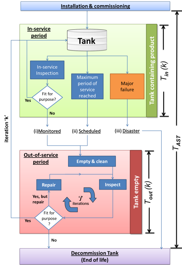
Figure 2: The AST life cycle: after the initial commissioning come 'k' iterative loops of in-service followed by out-of-service cycles which repeat until the tank is finally decommissioned. The operational lifetime of the AST is denoted by T_{AST} and the periodic in-service and out-of-service intervals at iteration 'k' are represented by T_{in}(k) and T_{out}(k) respectively.
